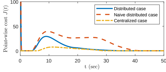
Fig. 6: Time evolution of the cost \sum_{i \in \mathcal{I}} \frac{1}{2} \|\mathbf{x}_i - \mathbf{x}_{nom,i}\|^2 along the state trajectory when the proposed algorithm is applied.
