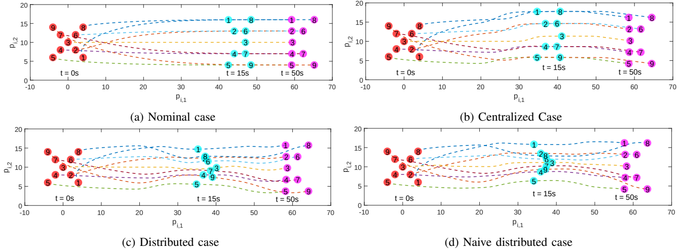
Fig. 4: Safe distributed control for coordinating 9 agents.
