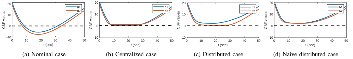
Fig. 5: Time evolution of the CBF values when coordinating 9 agents.
